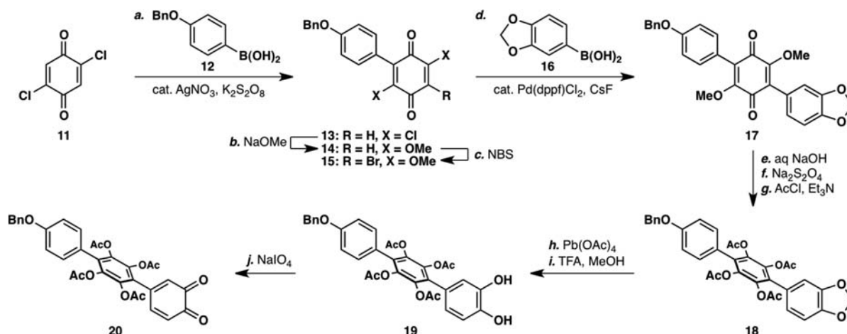
Scheme 2. Preparation of ortho-Quinone Heterodiene 20 a
