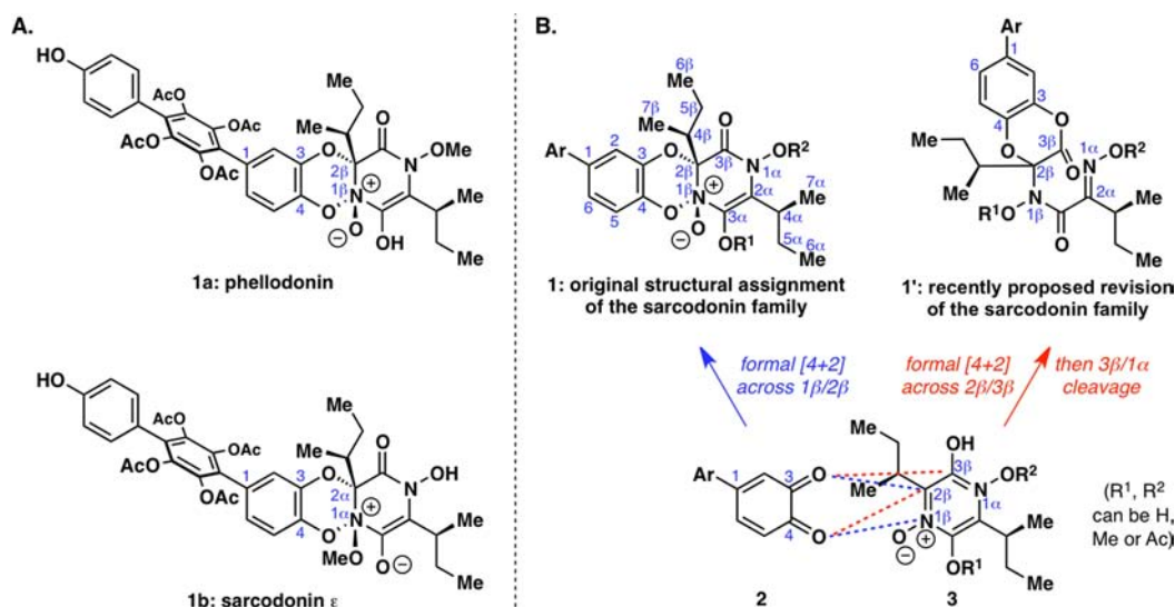
Figure 1. (A) Structures of recently isolated natural products, phellodonin ( 1a ) and sarcodonin ε ( 1b ). (B) Originally published structure for the sarcodonin family ( 1 ) and our recently proposed structure revision ( 1' ), both arising from a hypothetical biosynthesis via a formal [4 + 2] cycloaddition of ortho-quinone 2 and pyrazine derivative 3 .
