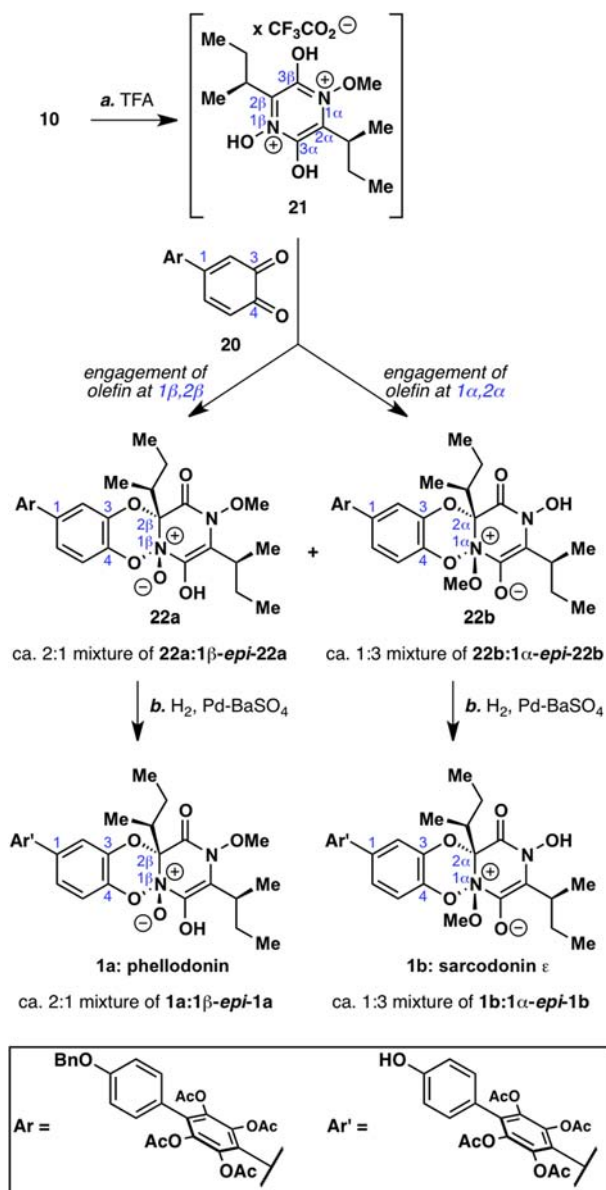
Scheme 3. Formal Hetero-Diels–Alder Reaction for the Synthesis of Phellodonin ( 1a ) and Sarcodonin \epsilon ( 1b ) a
